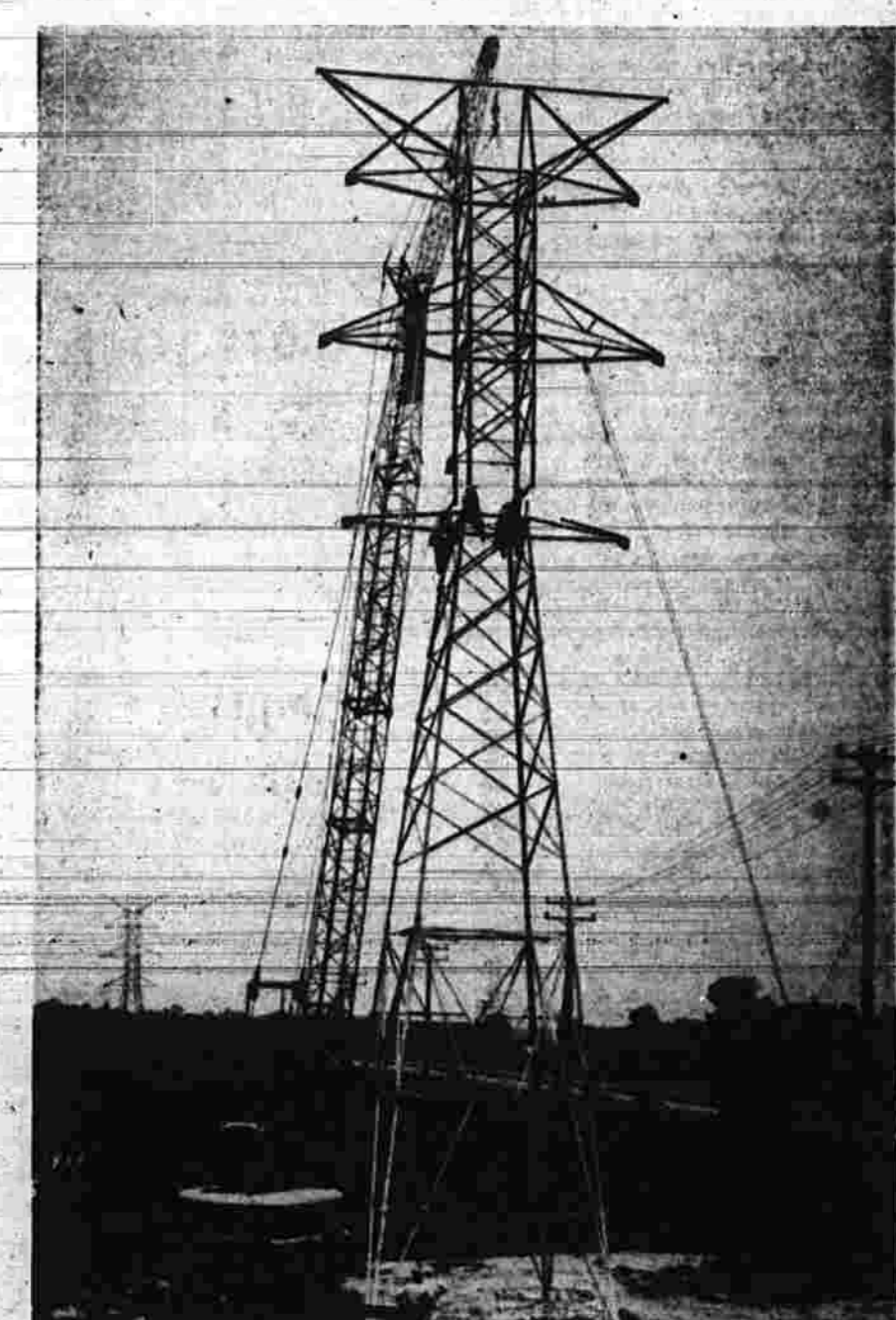
Top Section of Tower being lowered into place on the Wilbur Cross Highway near Forbes Street in East Hartford. The wood pole line carries the two 22,000 volt circuits which previously supplied Manchester and which are now used to carry power from the new 115,000 volt substation in Manchester, back to load centers in East Hartford.
