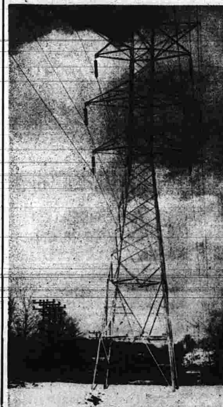
A straight away section of the two circuit 115,000 volt tower line. Each circuit consists of three phase wires and there are two wires on the top of the tower which protect against lightning.
